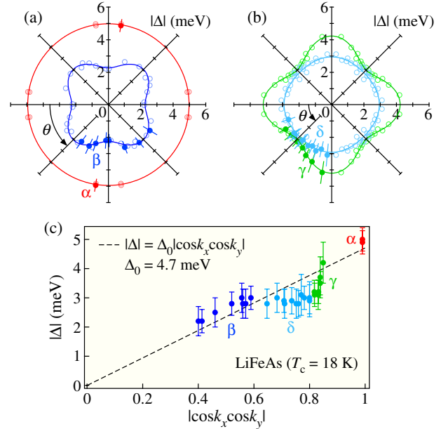
FIG. 4 (color online). (a) and (b) Polar plots of the SC gap size for the \alpha , \beta and the \gamma , \delta FSs, respectively, as a function of \theta defined in Fig. 3(a). Filled circles are the original data, and open circles are the folded data which take into account the fourfold symmetry. Error bars in (a)–(c) originate from the fitting uncertainty on \Delta , as well as experimental uncertainties in determining the energy position of E_F and the momentum location of k_F (less than 0.1 and 0.2 meV, respectively). Solid curves show the fitting results with \Delta(\theta) = \Delta_0 + \Delta_1 \cos[4(\theta + \phi)] . (c) Plot of the SC gap size as a function of |\cos k_x \cos k_y| . The fitting result assuming the gap function |\Delta| = \Delta_0 |\cos k_x \cos k_y| is indicated by a black dashed line.
