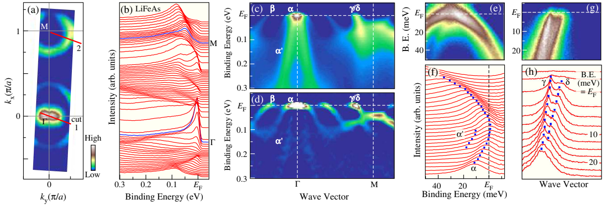
FIG. 1 (color online). (a) Plot of the ARPES intensity at E_F of LiFeAs ( T_c = 18 K) as a function of the two-dimensional wave vector measured with the He I\alpha line ( h\nu = 21.218 eV). The intensity is obtained by integrating the spectra within \pm 5 meV with respect to E_F . (b) ARPES spectra along the \Gamma - M high-symmetry line. (c) and (d) Intensity plot and second-derivative intensity plot of (b), respectively, as a function of binding energy and wave vector. (e) ARPES intensity plot at T = 50 K divided by a Fermi-Dirac function measured along cut 1 in (a), and (f) corresponding energy distribution curves. (g) ARPES intensity plot at 20 K along cut 2 and (h) corresponding momentum distribution curves. Blue dots in (f) and (h) are guides for the eye to trace the band dispersion.
